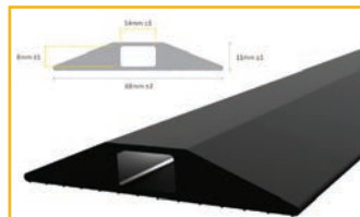
CablePRO GP - Black CP010012 & CP010005 Channel Size: 8mm W x 14mm H
