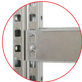
M50 Upright & C50 Beam
