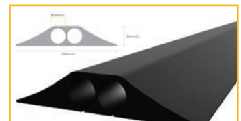
CablePRO HD - HD2 CP010009 & CP010002 2 x Channel Size: 230 mm
