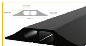
CablePRO Data CP010010 & CP010003 2 x Channel Size: Channel Size: 15mm W x 10mm
