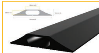
CablePRO GP - Black CP010013 & CP010006 Channel Size: 30mm W x 10mm H
