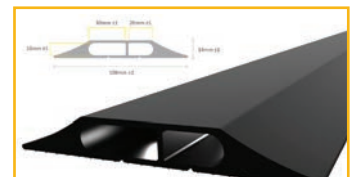
CablePRO Data CP010011 & CP010004 2 x Channel Size: 30mm W x 10mm H & 20mm W x 10mm H
